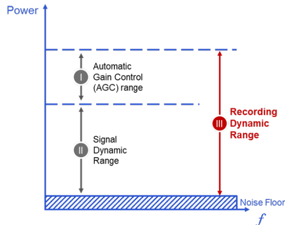
Figure 3 Dynamic Range
